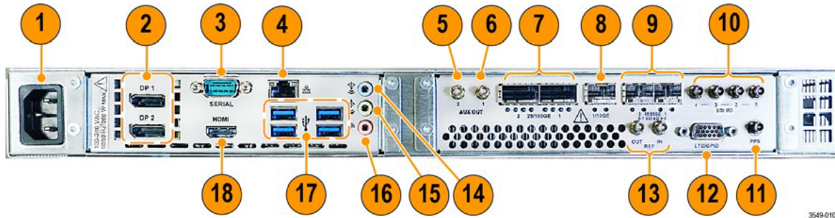
Descriptions of numbered PRISM MPX2-25 rear-panel connectors
