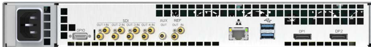
Labeled PRISM MPP-100 Rear-Panel Connectors
