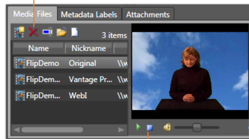
Mini-player controls.
